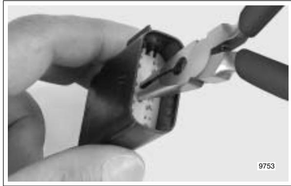
Figure B-42. Pull Up Secondary Lock (Pin Housing)
