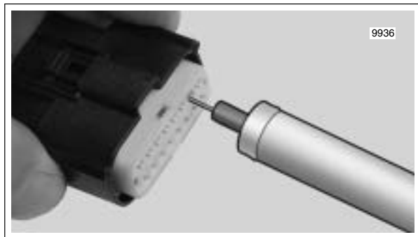
Figure B-44. Insert Molex Connector Terminal Remover (Part No. HD-48114)
