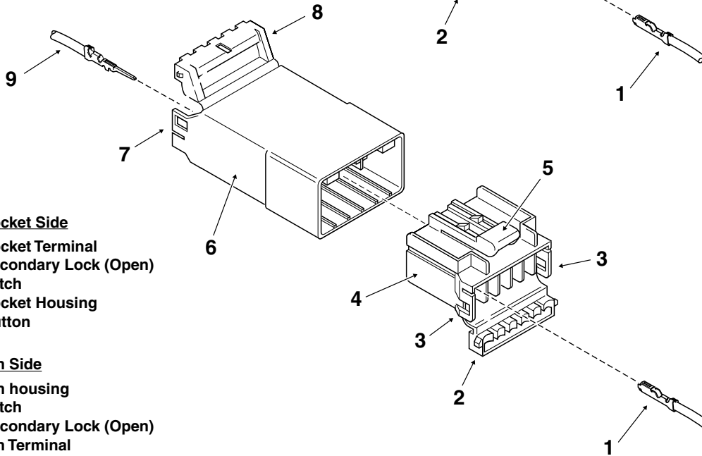
Figure B-14. 3-Place and 6-Place Multilock Connectors
