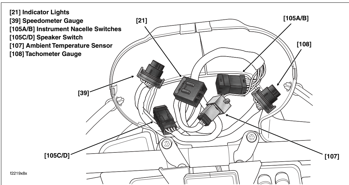
Figure B-56. Instrument Nacelle Connectors (FLTR)
