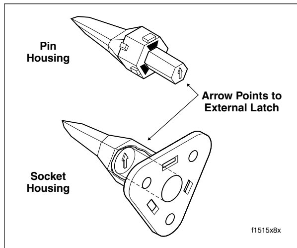
Figure B-4. 3-Place Locking Wedge Orientation
