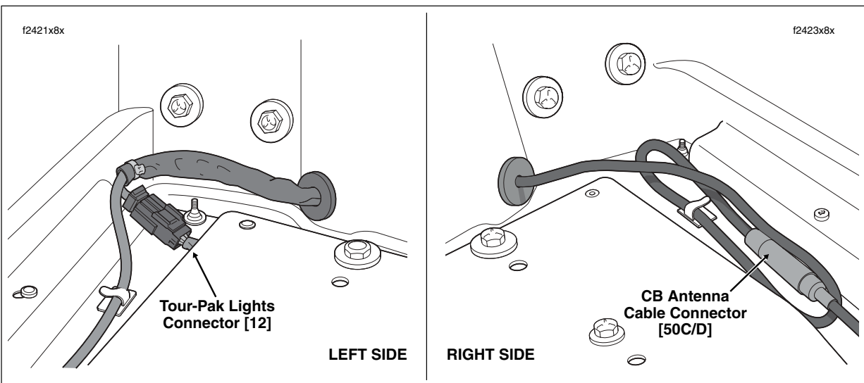
Figure B-51. Tour-Pak Connectors
