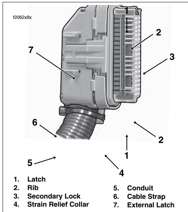
Figure B-33. Remove Secondary Lock
