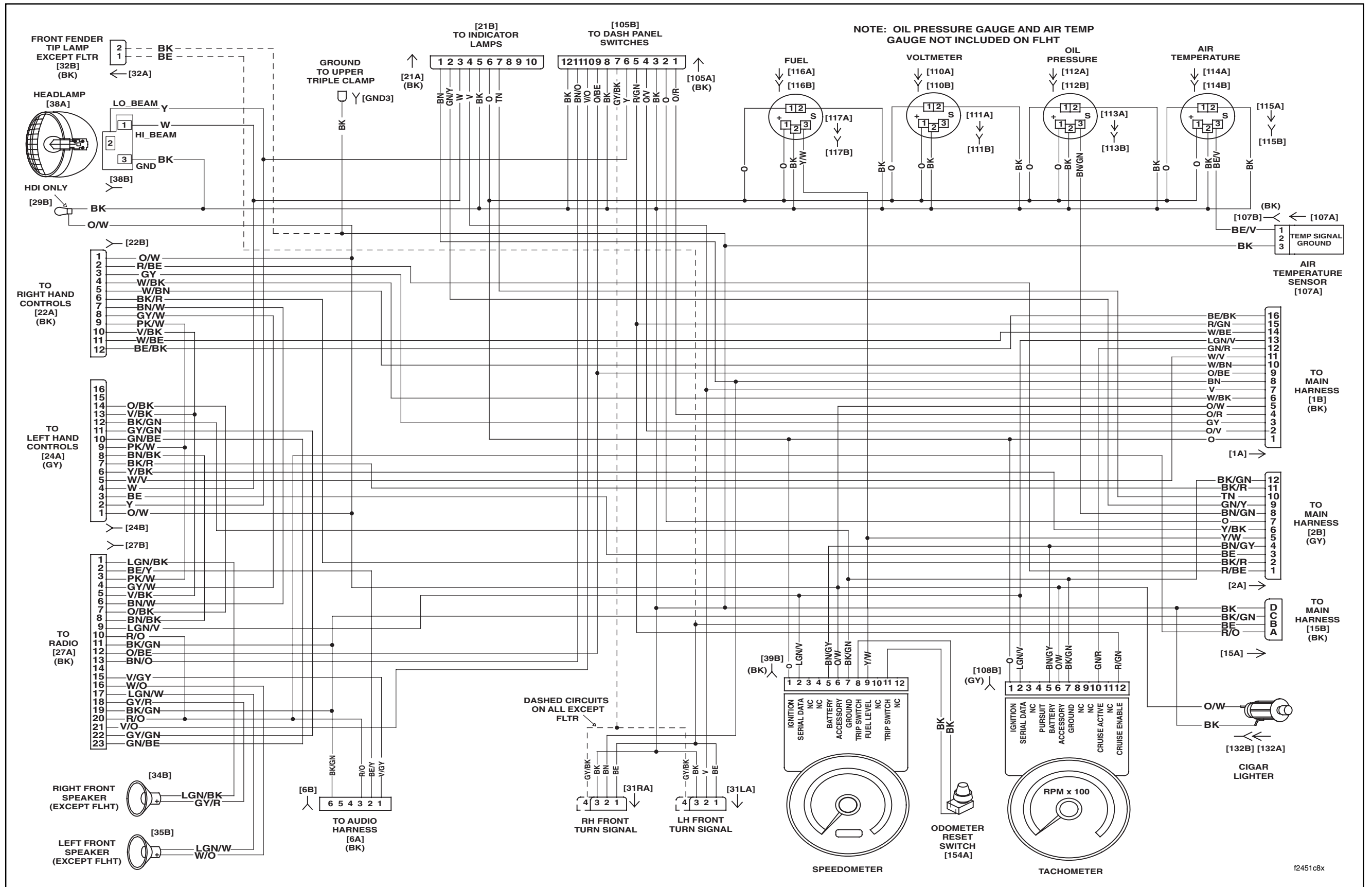
2007 FLHX, FLHT, FLHTC, FLHTCU and FLTR, DOMESTIC and INTERNATIONAL Models, Interconnect Harness
