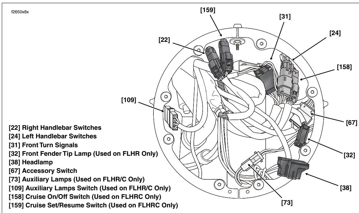
Figure B-58. Headlamp Nacelle Connectors (FLHR/C/S)
