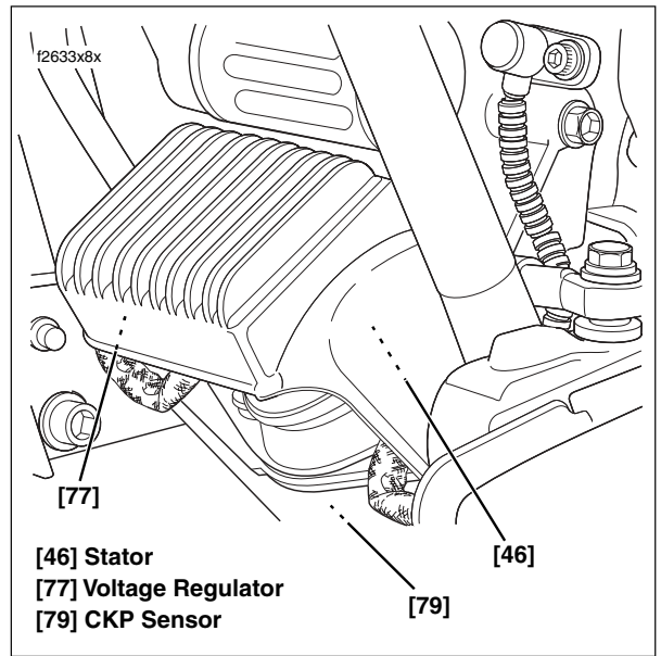
Figure B-54. Voltage Regulator (Left Side View)
