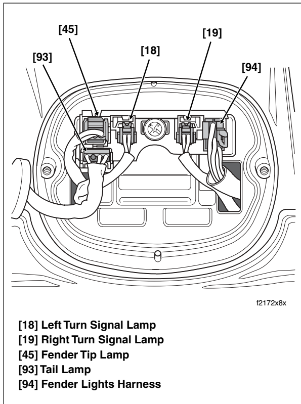
Figure B-53. Rear Fender Lights Assembly
