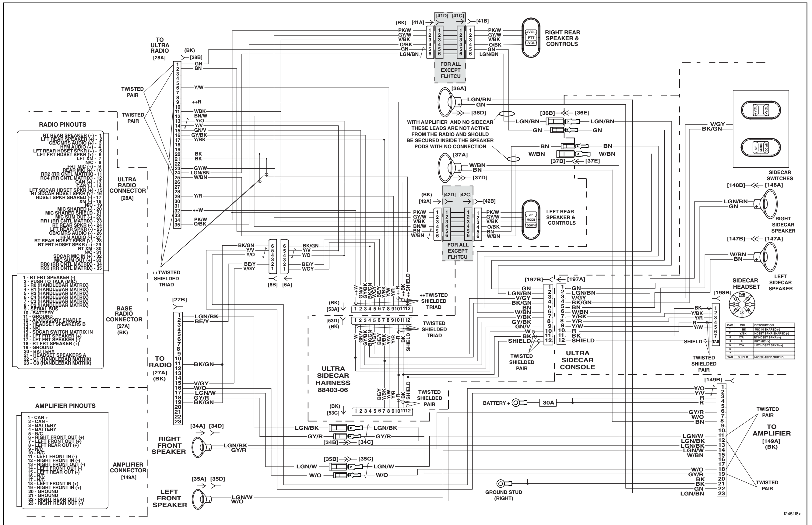
2007 TLE, TLE-U SIDECARS, DOMESTIC AND INTERNATIONAL Models, Amplifier, Sidecar Speakers and Switches
