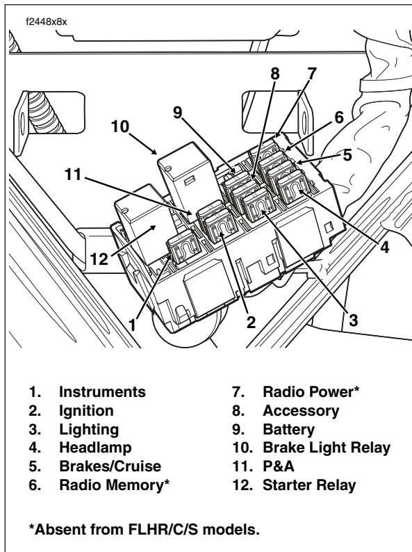
Figure B-48. Fuse Blocks - FLHX, FLHTC/U, FLTR (Under Left Side Cover)
