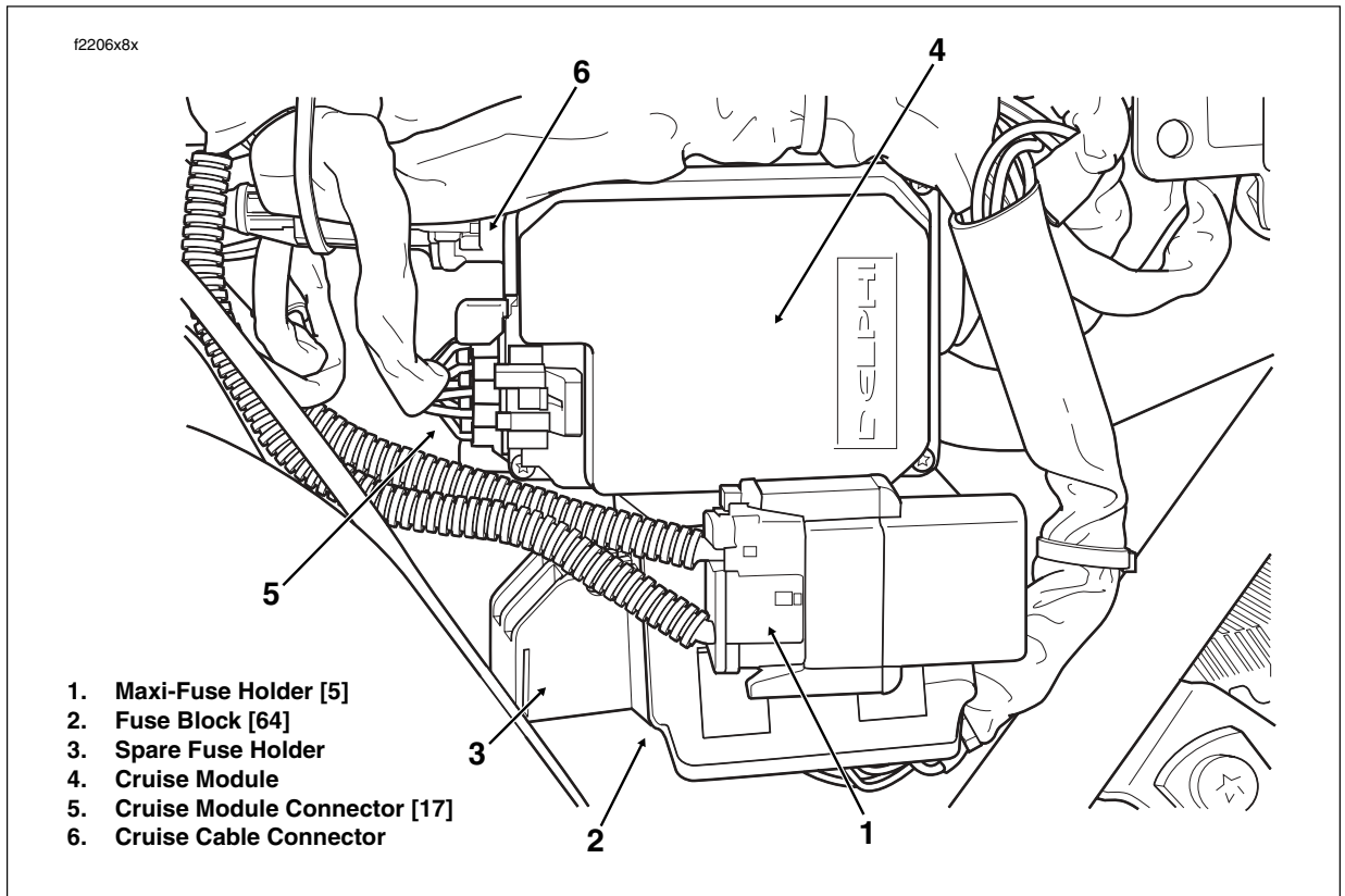
Figure B-47. Cruise Control Module (Under Left Side Cover)
