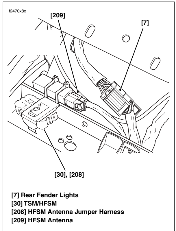
Figure B-55. Rear Fender (Under Seat)
