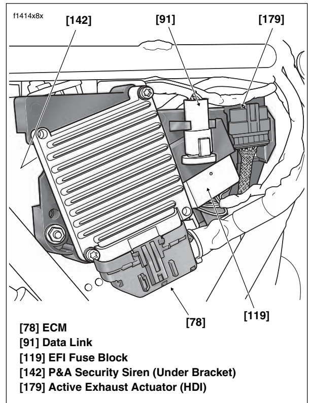
Figure B-49. Under Right Side Cover
