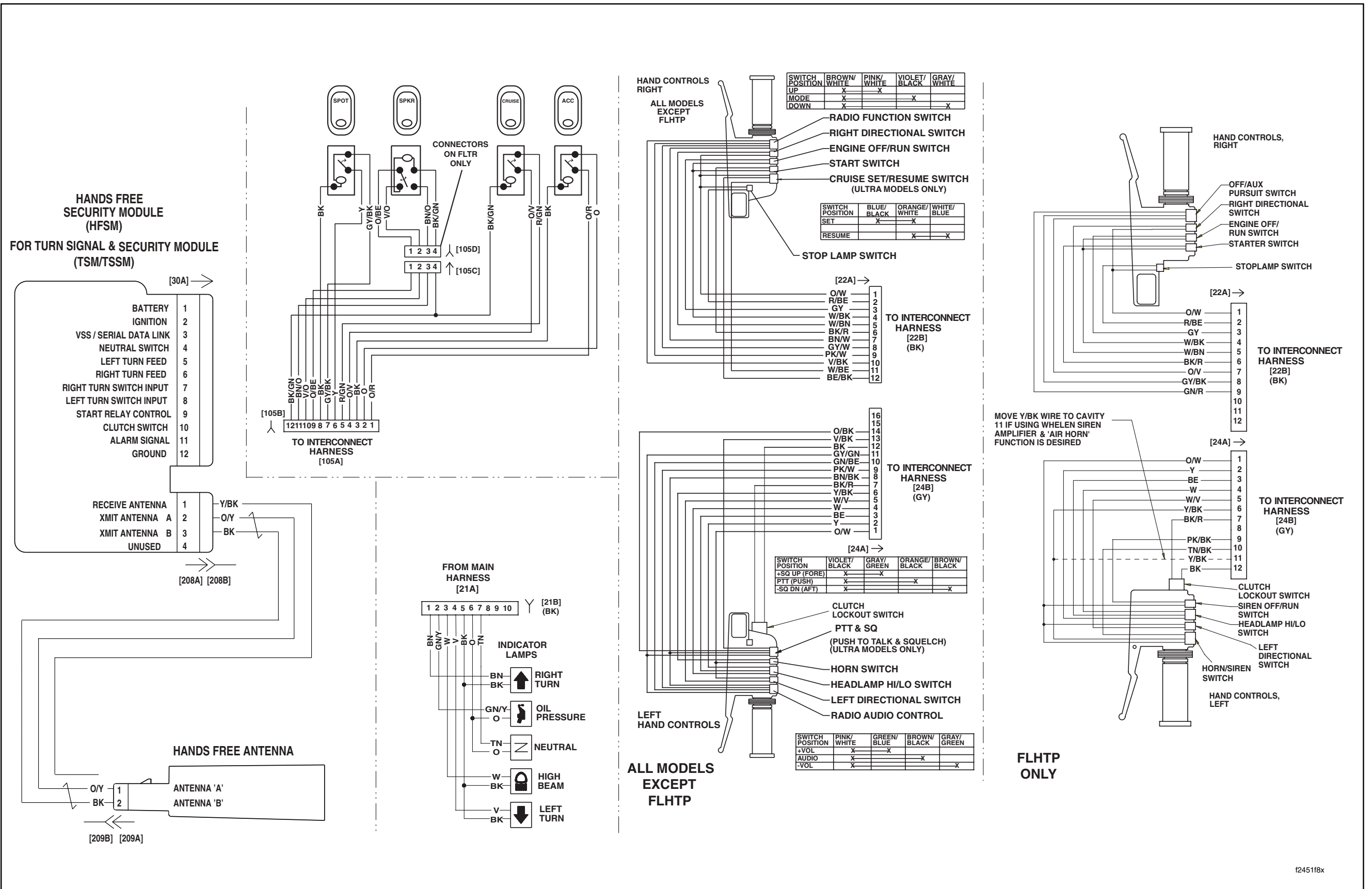
2007 FLHX, FLHT, FLHTC, FLHTCU and FLTR, DOMESTIC and INTERNATIONAL Models, Handlebar Switches, Indicator Lamps, Fairing Cap/Instrument Nacelle Switches and HFSSM/Antenna
