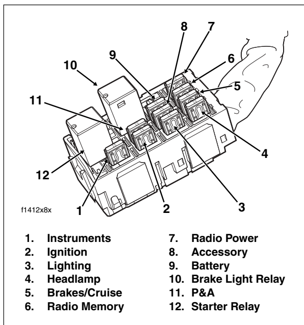
Figure B-22. Fuse Block (FLHX, FLHTC/U, FLTR)
