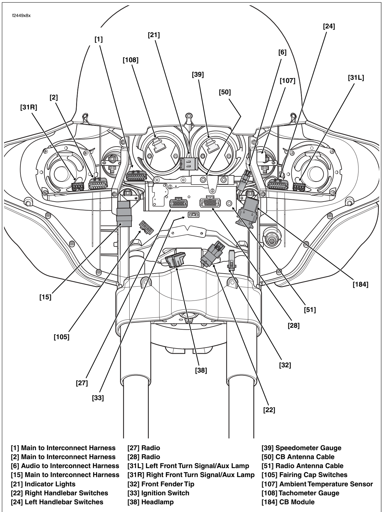
Figure B-46. Inner Fairing Connectors (FLHX, FLHT/C/U)
