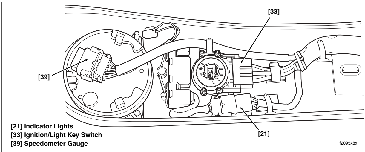
Figure B-59. Instrument Console Connectors (FLHR/C)
