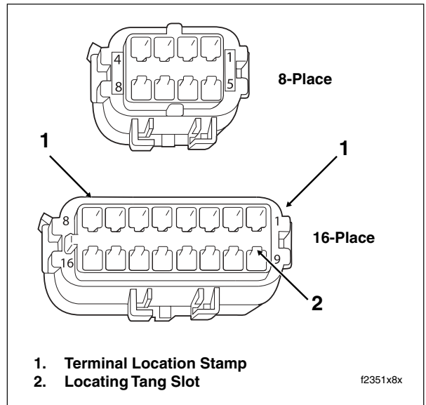
Figure B-45. Wire End (Pin Housing Shown)
