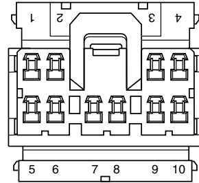
10-Place Connector
