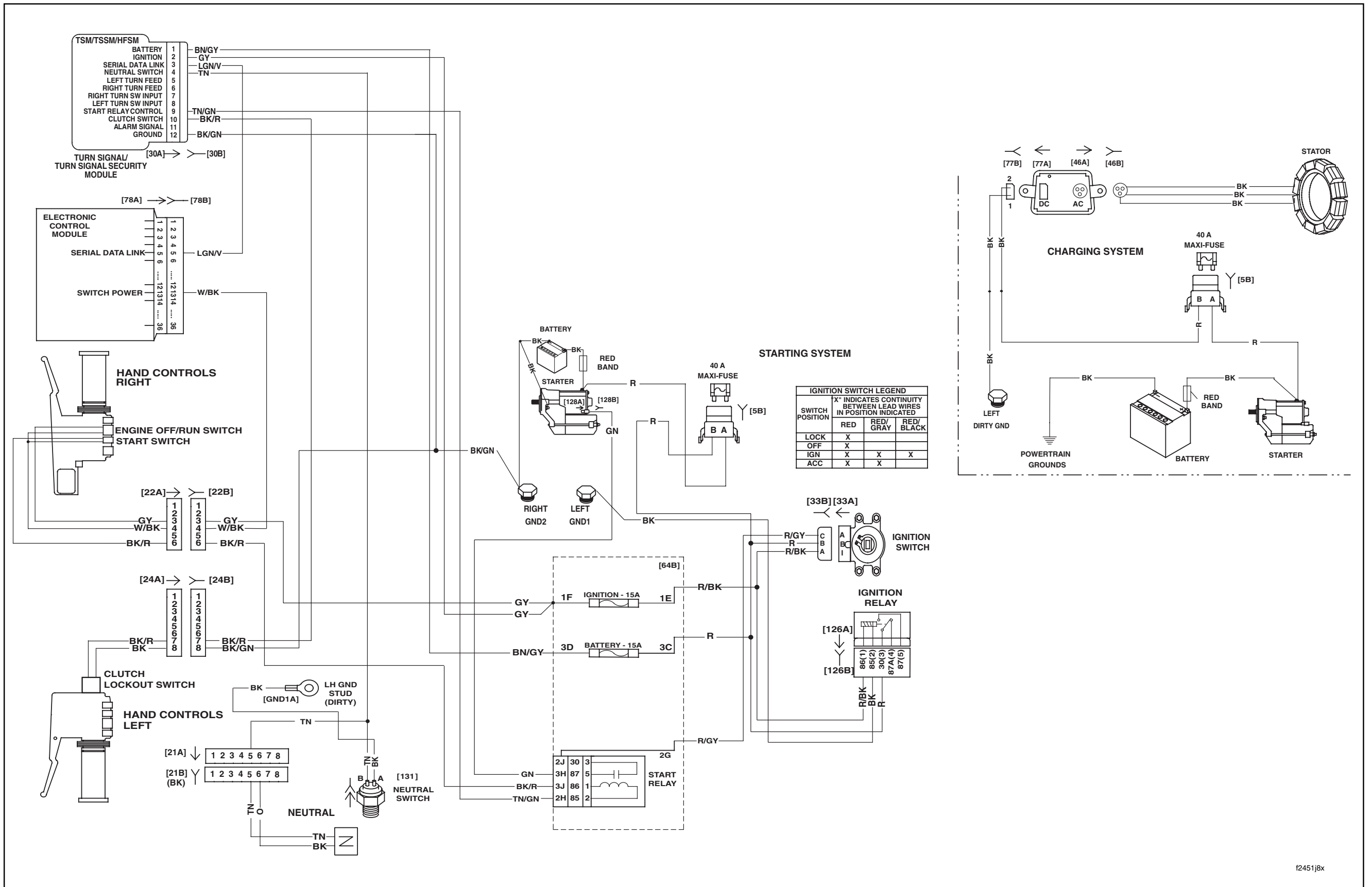
2007 FLHR, FLHRC and FLHRS, DOMESTIC and INTERNATIONAL Models, Starting and Charging
