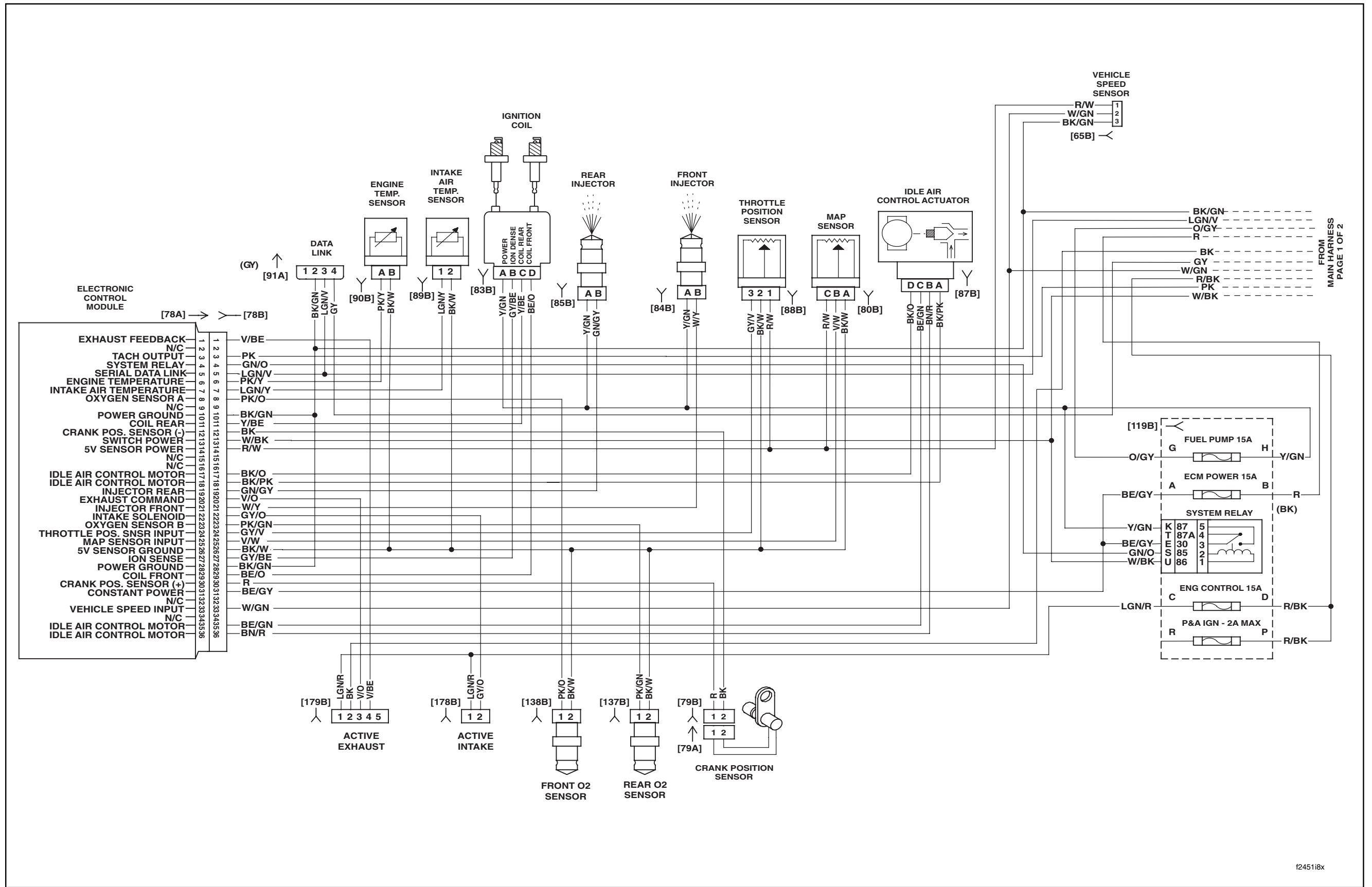
2007 FLHR, FLHRC and FLHRS, DOMESTIC and INTERNATIONAL Models, Main Harness (Page 2 of 2)
