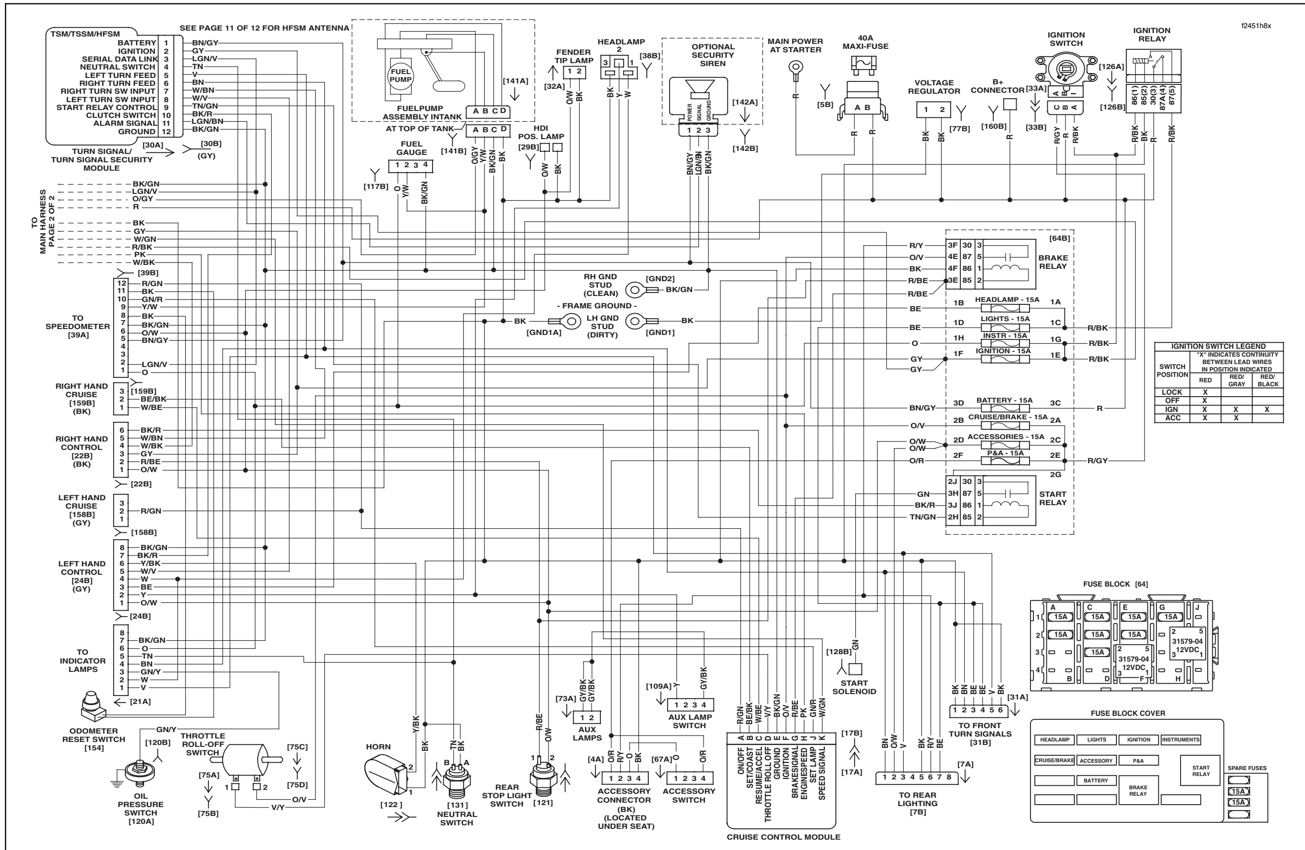
2007 FLHR, FLHRC and FLHRS, DOMESTIC and INTERNATIONAL Models, Main Harness (Page 1 of 2)
