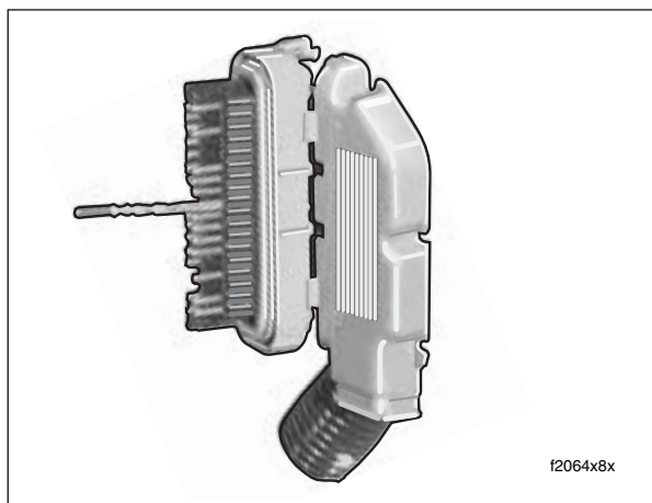
Figure B-35. Push Wire to Extract Terminal
