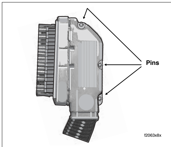
Figure B-34. Separate Halves of Socket Housing
