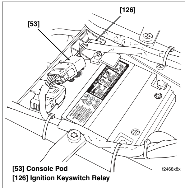
Figure B-52. Frame Crossmember (Under Seat)
