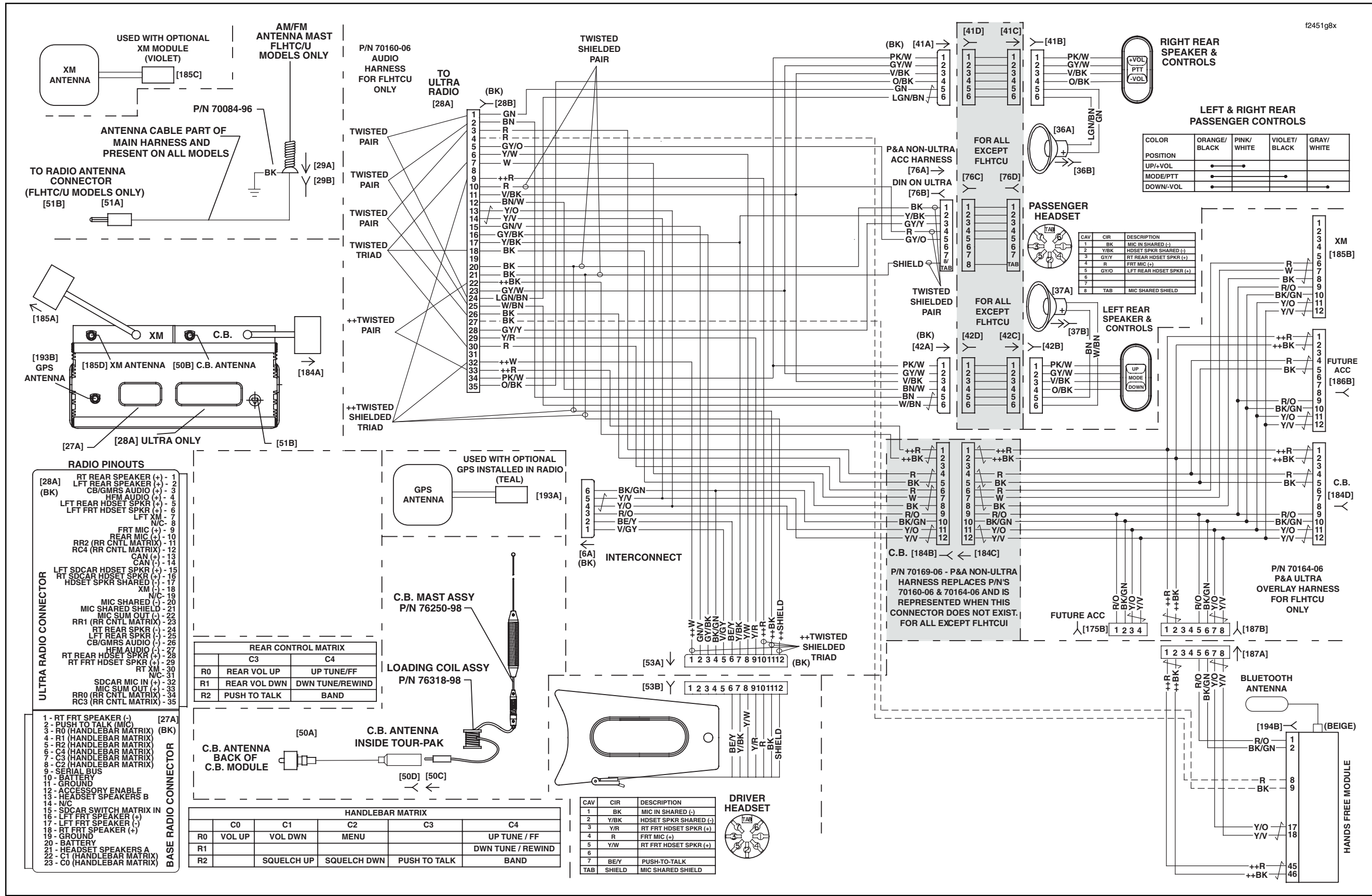
2007 FLHX, FLHTC, FLHTCU and FLTR, DOMESTIC and INTERNATIONAL Models, Radio, CB/Intercom, Rear Speakers, XM, Hands Free Phone and Navigation
