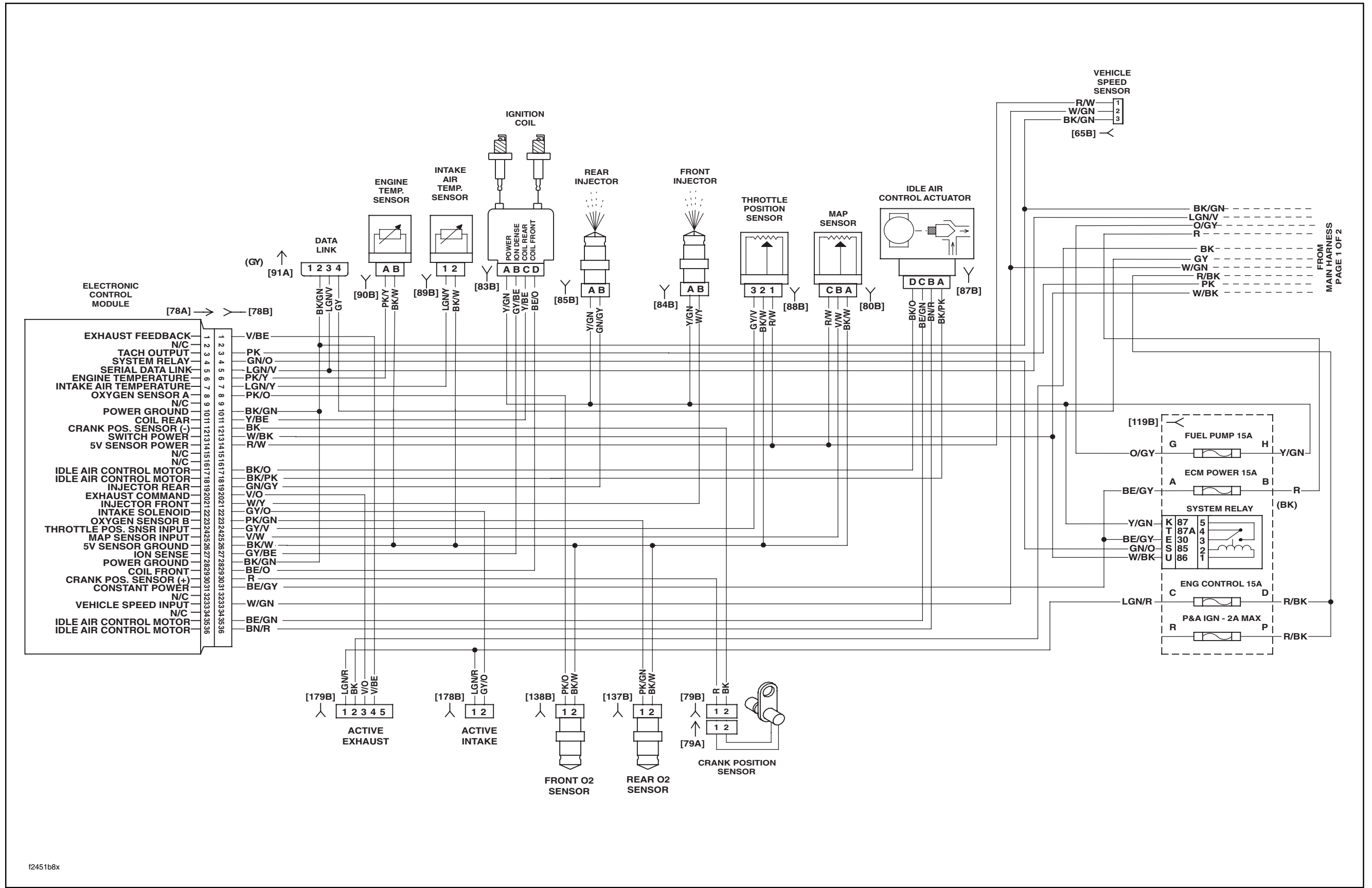
2007 FLHX, FLHT, FLHTC, FLHTCU and FLTR, DOMESTIC and INTERNATIONAL Models, Main Harness (Page 2 of 2)
