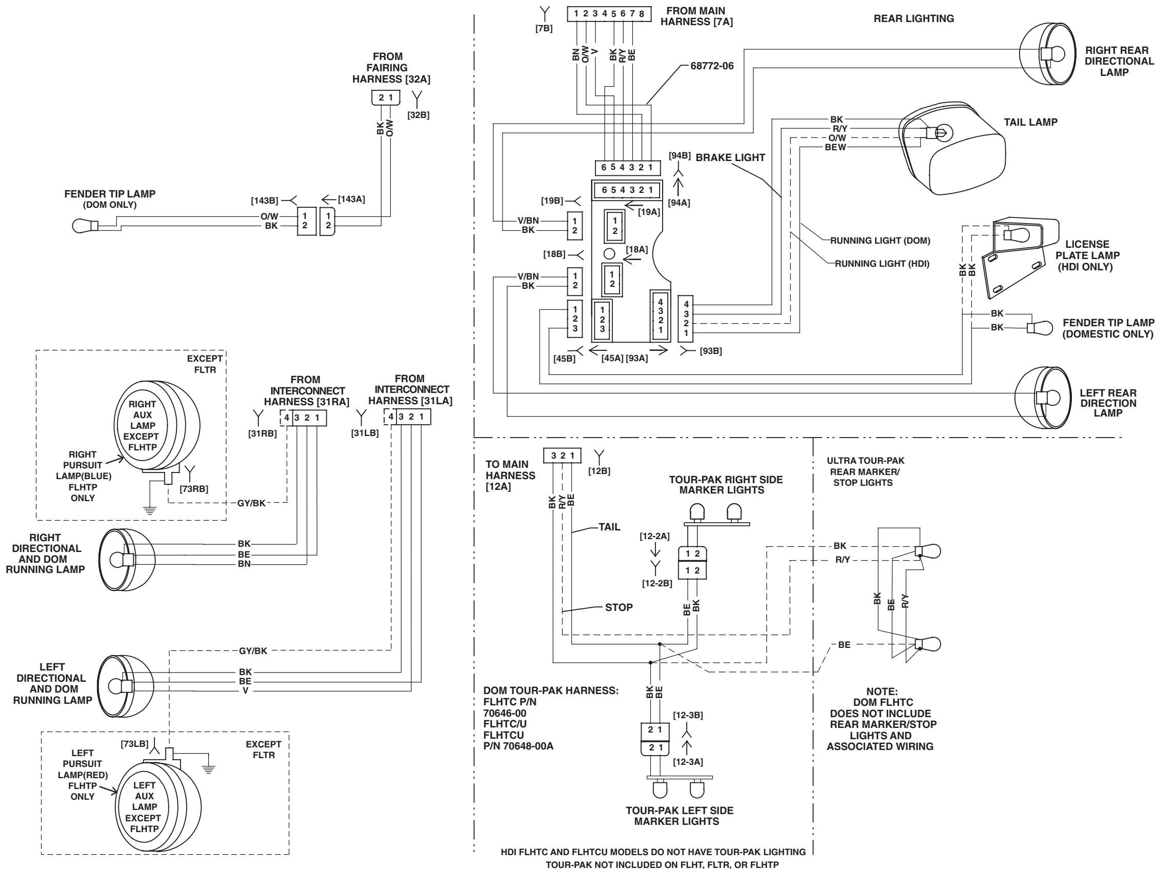
2007 FLHX, FLHT, FLHTC, FLHTCU and FLTR, DOMESTIC and INTERNATIONAL Models, Tail Lamp, Auxiliary Lamps, Fender Tip Lamps, Directional Lamps and Tour-Pak Lights
