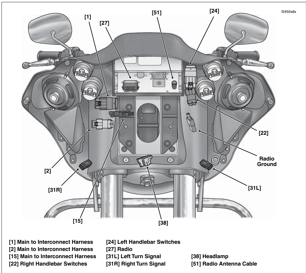
Figure B-57. Inner Fairing Connectors (FLTR)
