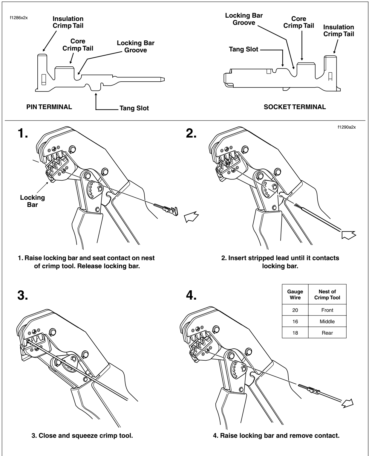
Figure B-15. Multilock Crimping Procedure
