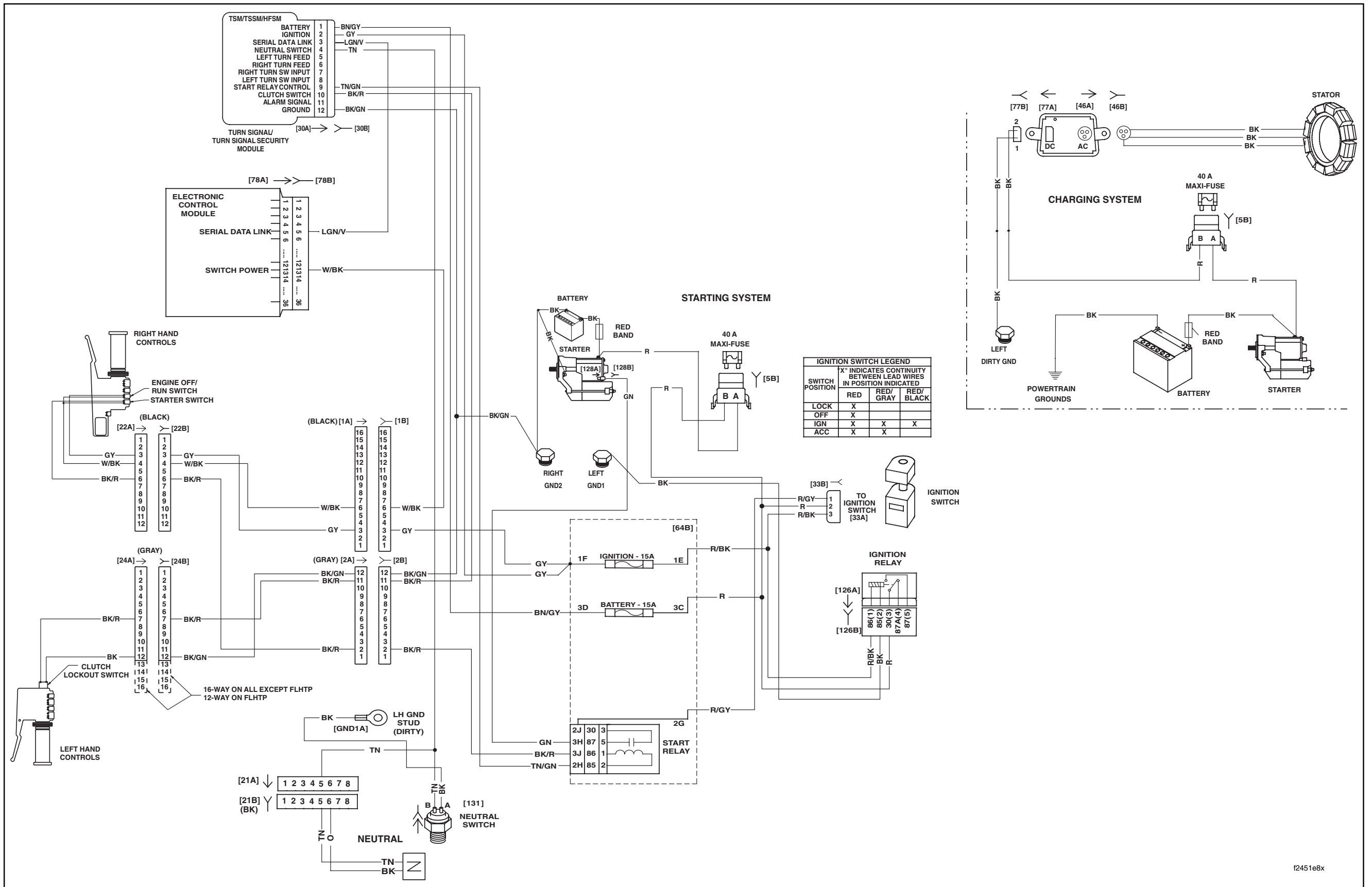
2007 FLHX, FLHT, FLHTC, FLHTCU and FLTR, DOMESTIC and INTERNATIONAL Models, Starting and Charging
