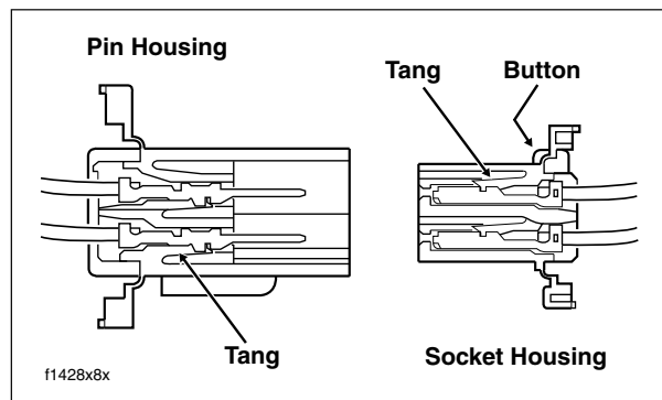
Figure B-12. Tang Location (Cross Sectional View)
