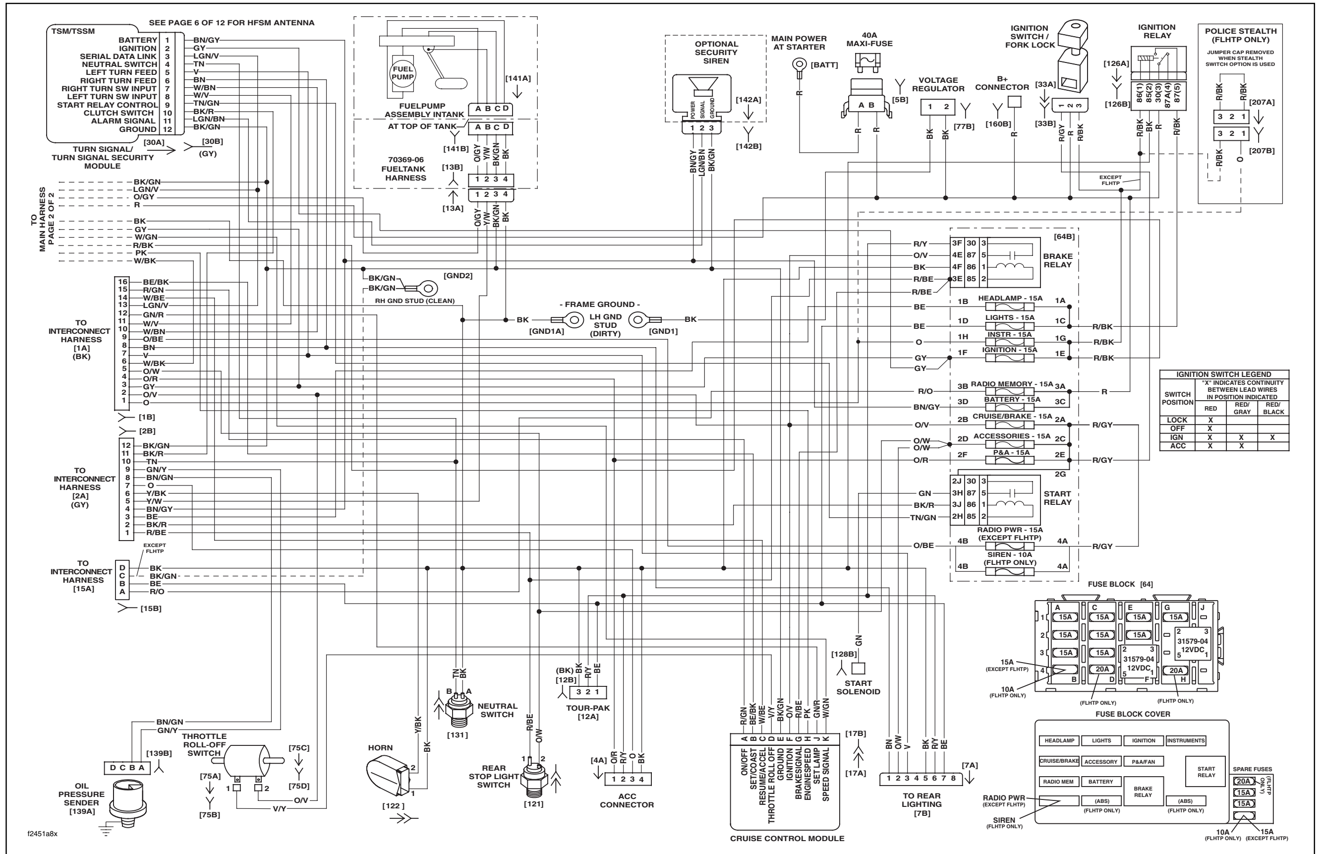
2007 FLHX, FLHT, FLHTC, FLHTCU and FLTR, DOMESTIC and INTERNATIONAL Models, Main Harness (Page 1 of 2)
