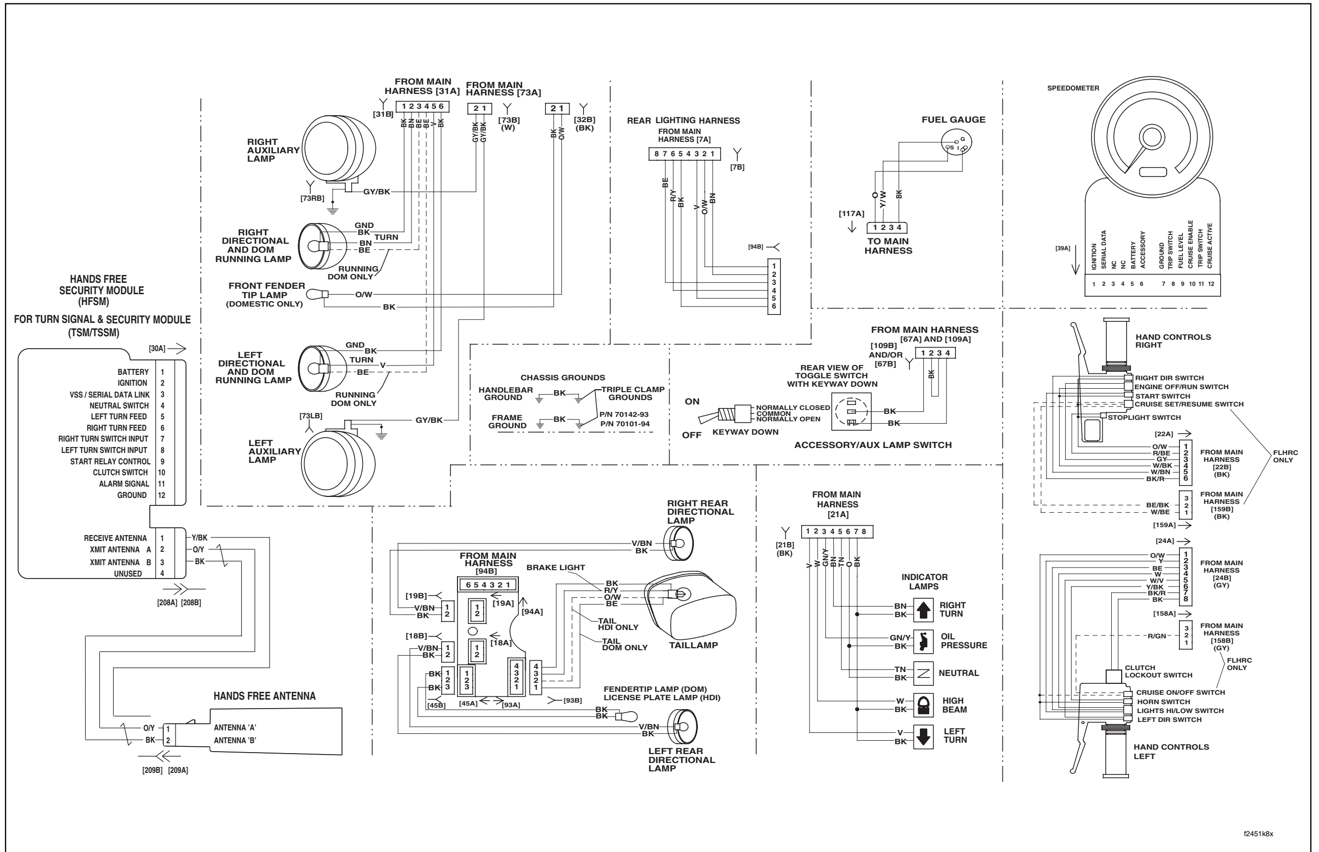
2007 FLHR, FLHRC and FLHRS, DOMESTIC and INTERNATIONAL Models, Handlebar Switches, Speedometer, Indicator Lamps, Tail Lamp, Auxiliary Lamps, Directional Lamps, Fender Tip Lamps and Aux Lamp/Accessory Switches B-65
