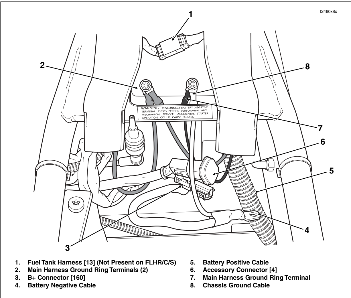
Figure B-50. Electrical Connectors - Upper Frame Crossmember (Under Seat)
