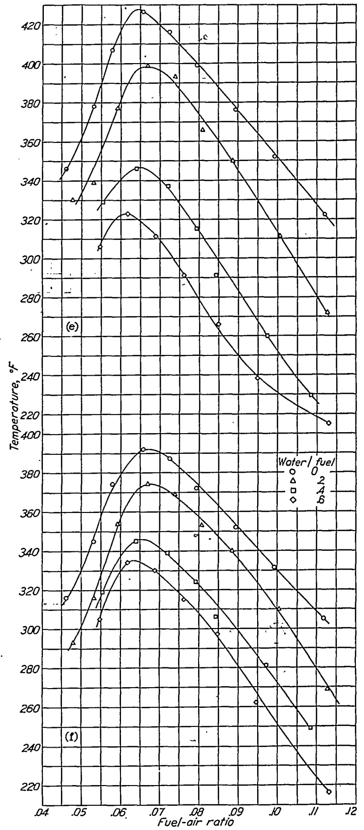
FIGURE 7.—Effect of water injection on engine temperature at constant manifold inlet pressure. Cylinder displacement, 202 cubic inches; engine speed, 2000 rpm; spark advance, 20°; compression ratio, 7.0; inlet-air temperature, 250° F; cooling pressure drop, 8.5 inches water; fuel, AFD-23; manifold inlet pressure, 35.0 inches of mercury absolute.
